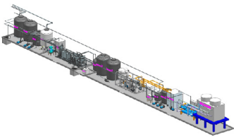
Acid Recovery Equipment and System
